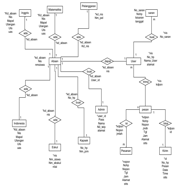
Gambar 2 ERD (Entity Relationship Diagram)
