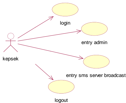
Gambar 1 Usecase Diagram
