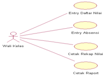
Gambar 4.13 Use Case Diagram Package Wali Kelas
