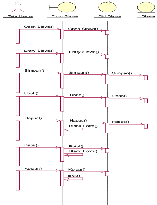
Gambar 4.32 Sequence Diagram Data Siswa
