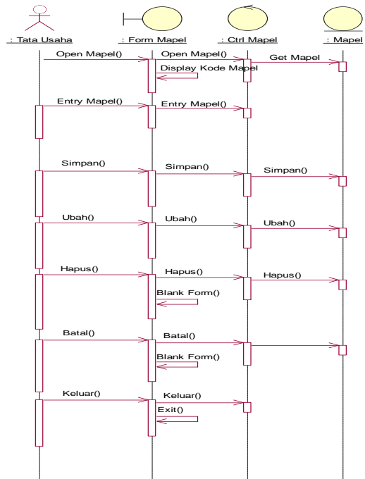
Gambar 4.34 Sequence Diagram Entry Mata Pelajaran
