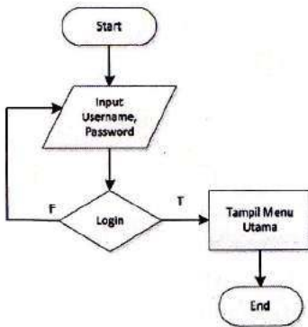
Gambar 3.17 Flowchart Login
